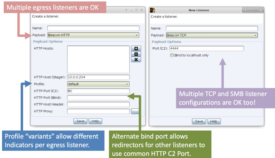
figure 35 - Infrastructure Consolidation Features
