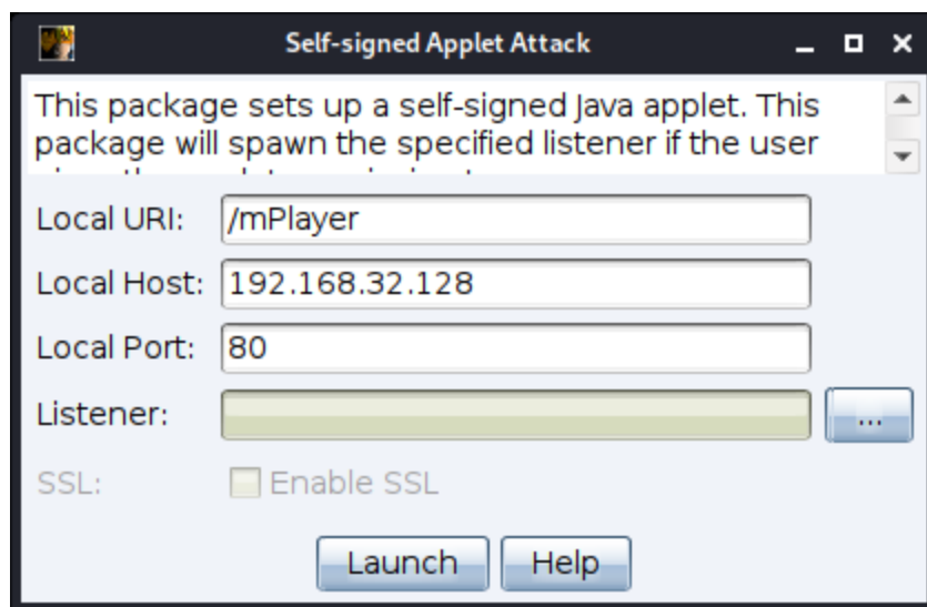
figure 45 - Signed Applet Attack
