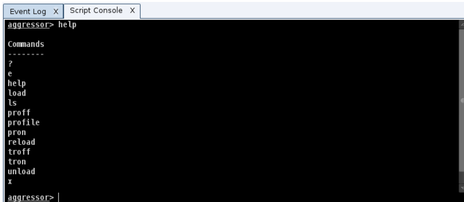
figure 70 - Interacting with the script console
