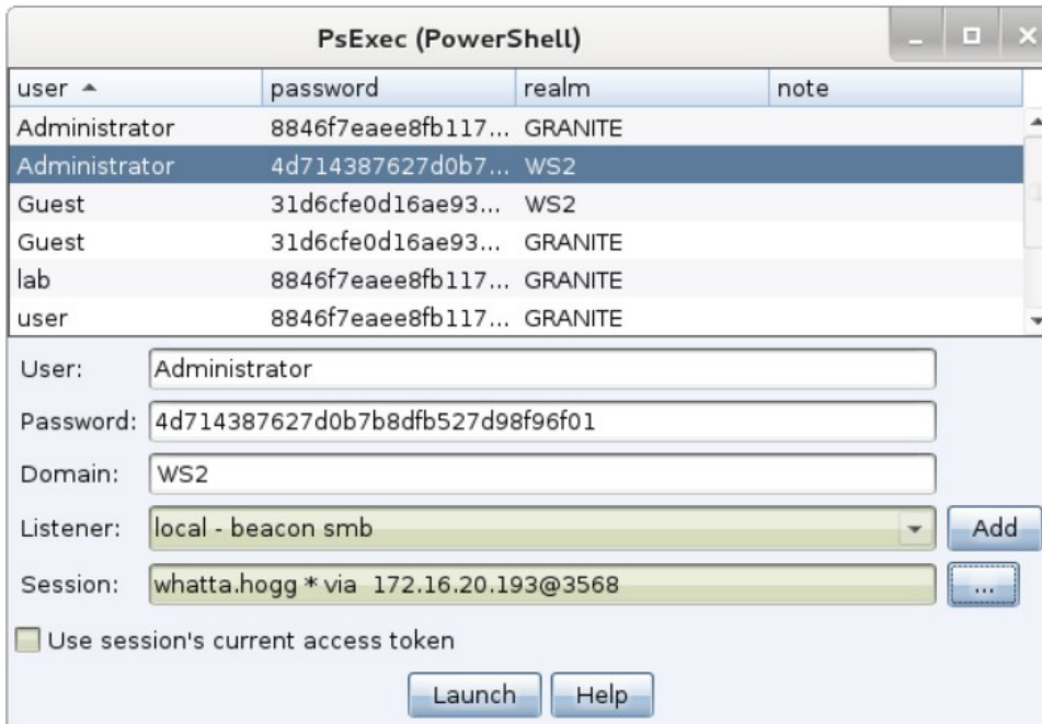
figure 60 - Lateral Movement Dialog
