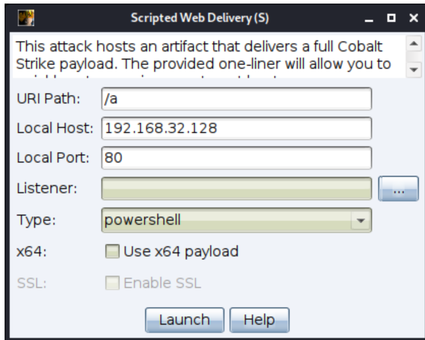
figure 47 - Scripted Web Delivery (S)
