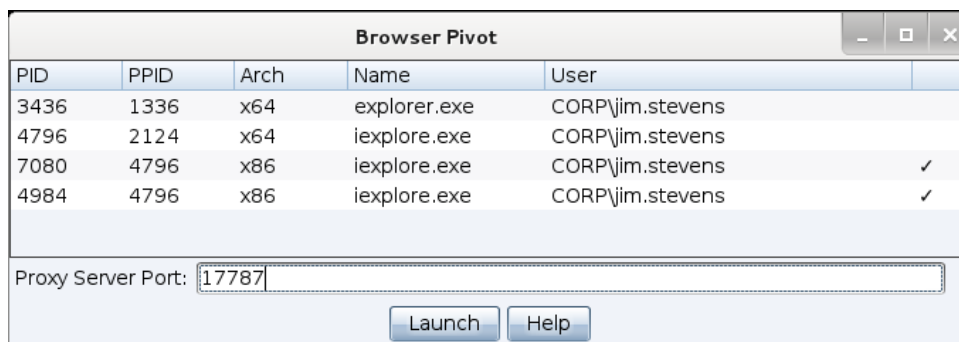
figure 62 - Start a Browser Pivot
