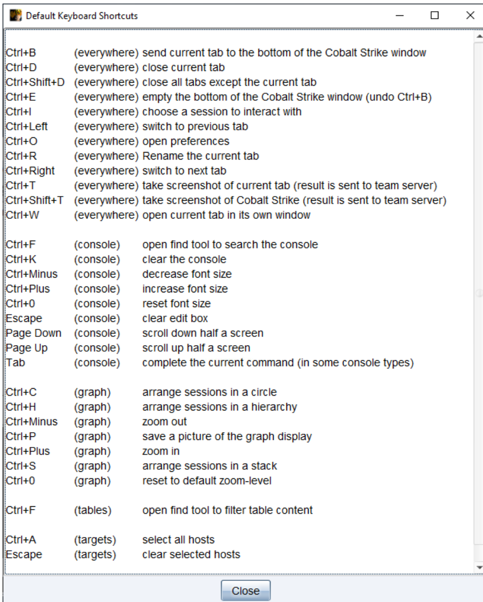
figure 17 - Default Keyboard Shortcuts
