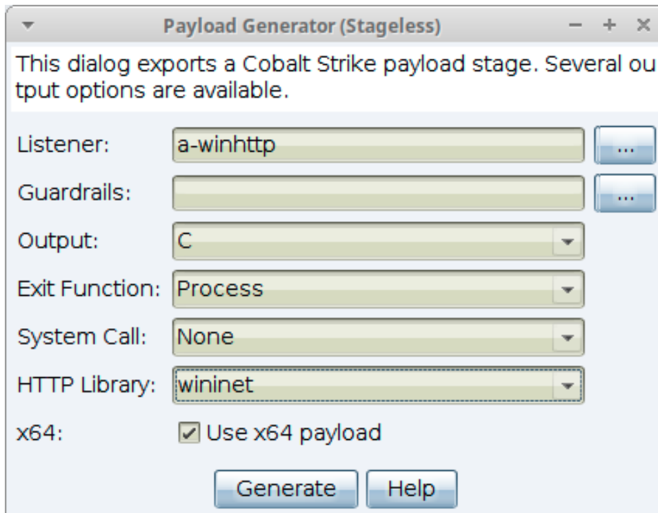
figure 39 - Stageless Payload Generator
