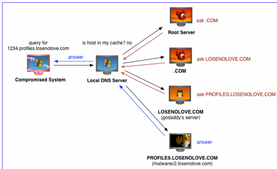
figure 23 - DNS Beacon in Action
