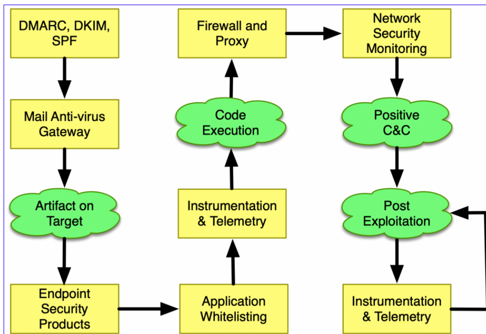
figure 1 - The Offense Problem Set
