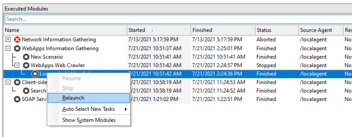
figure 49 - Executed Modules Panel - Relaunch Module
