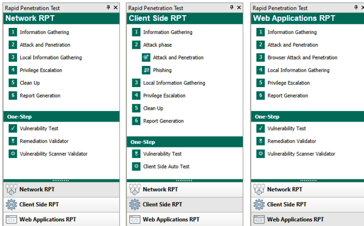
figure 9 - The Network RPT, Client Side RPT and Web Applications RPT Panels
