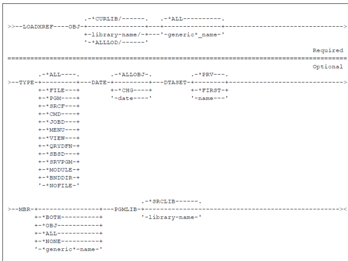
figure 8 - LOADXREF Command Diagram
