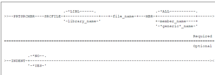
figure 50 - PRTSRCMBR Command Diagram
