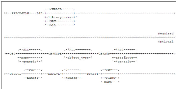
figure 55 - PRTOBJFLW Command Diagram
