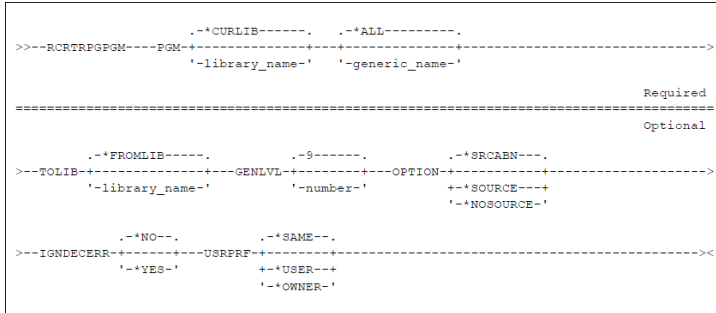
figure 42 - RCRTRPGPGM Command Diagram
