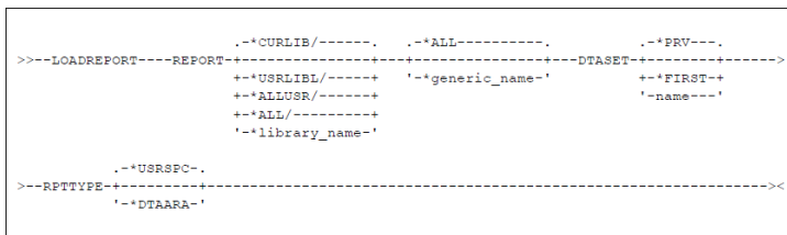
figure 15 - LOADREPORT Command Diagram
