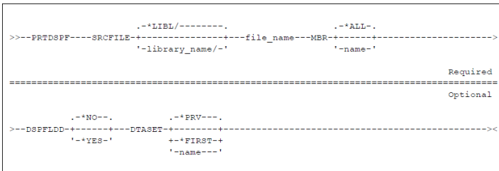
figure 37 - PRTDSPF Command Diagram
