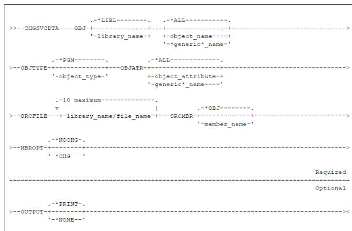
figure 52 - CHGSVCDTA Command Diagram
