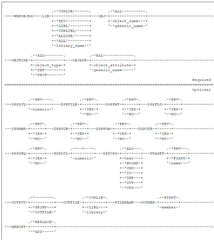
figure 29 - WRKOBJRX Command Diagram
