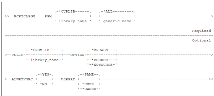
figure 44 - RCRTCLPGM Command Diagram
