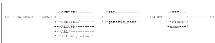
figure 13 - LOADMENU Command Diagram
