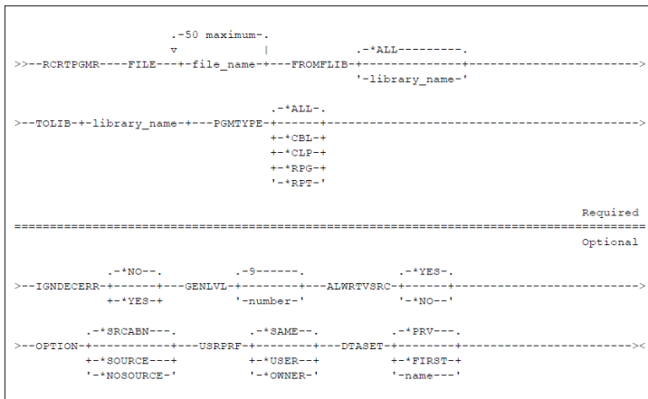
figure 41 - RCRTPGMR Command Diagram
