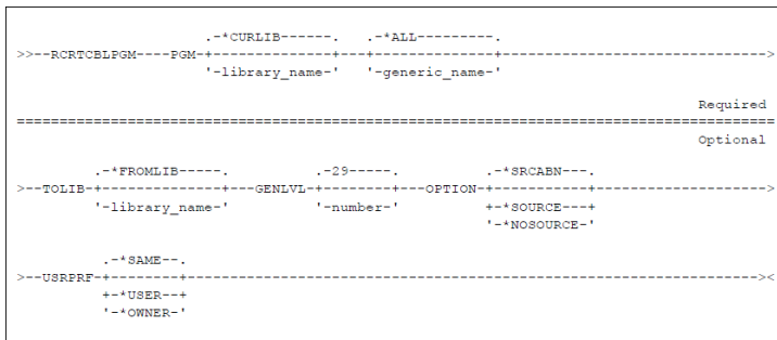
figure 43 - RCRTCBLPGM Command Diagram
