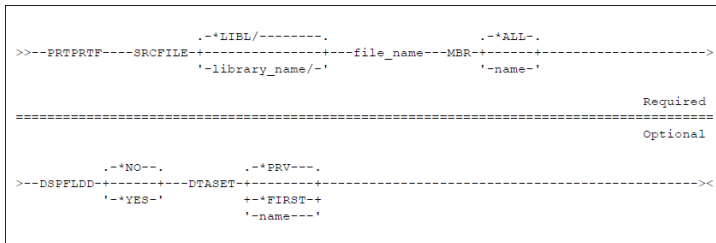
figure 36 - PRTPTF Command Diagram
